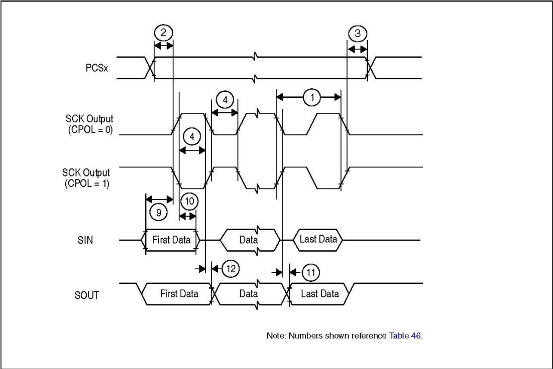
Figure 23. DSPI classic SPI timing — master, CPHA = 1
