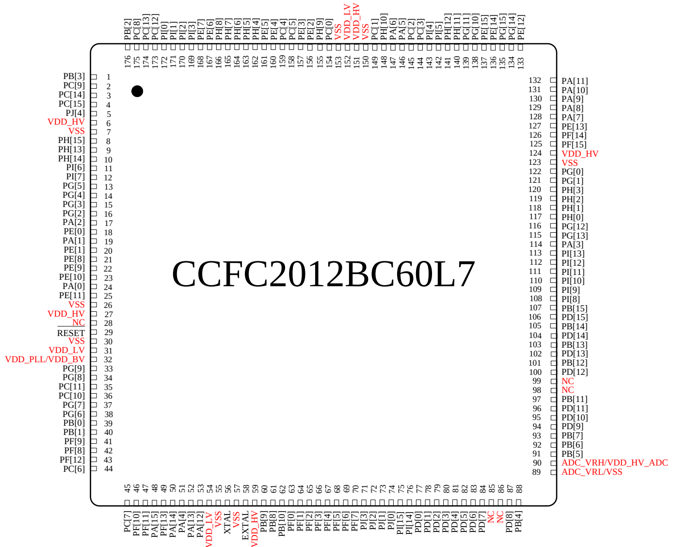
Figure 2. CCFC2012BC60L7 176 LQFP pin configuration
