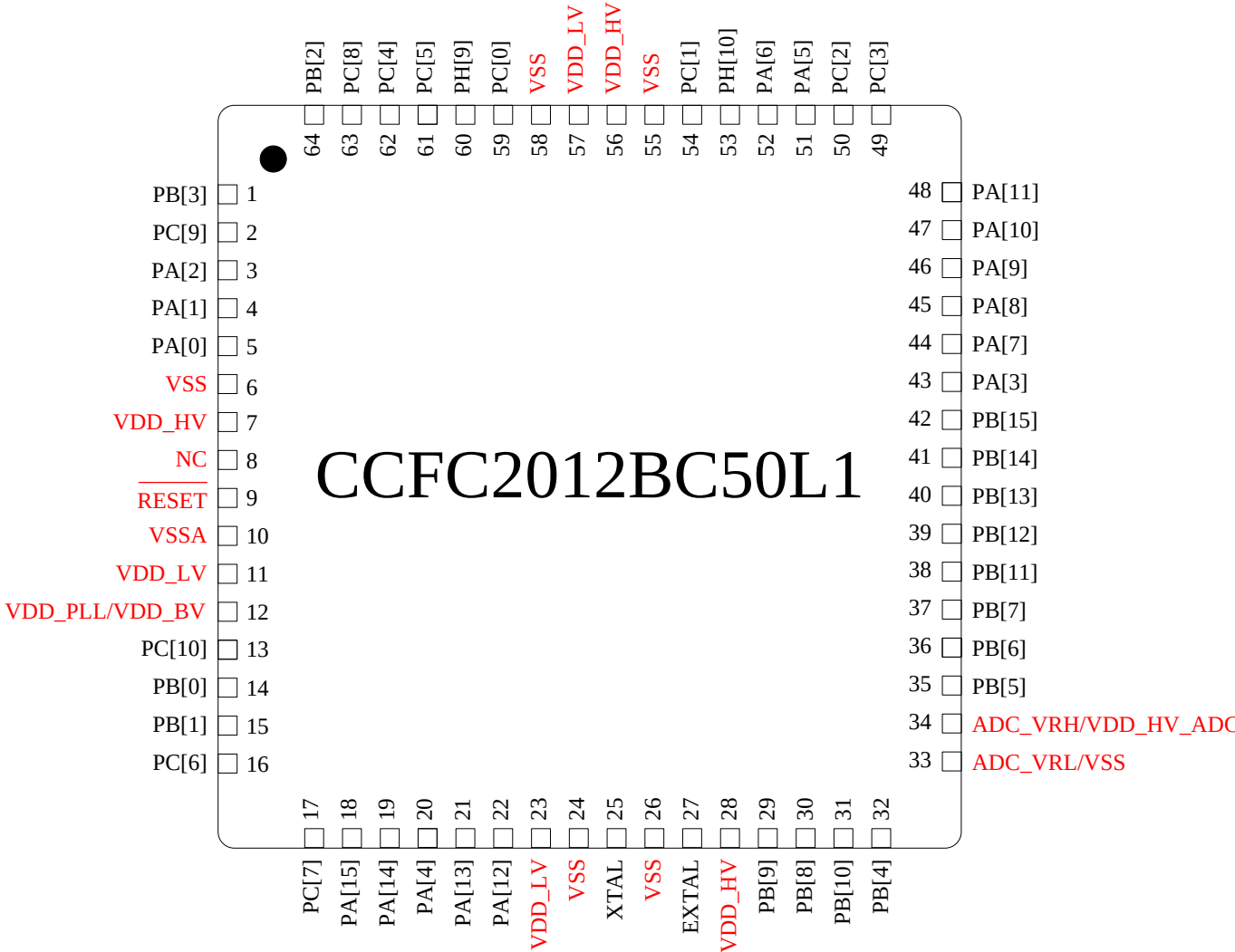
Figure 5 CCFC2012BC50L1 64 LQFP pin configuration
