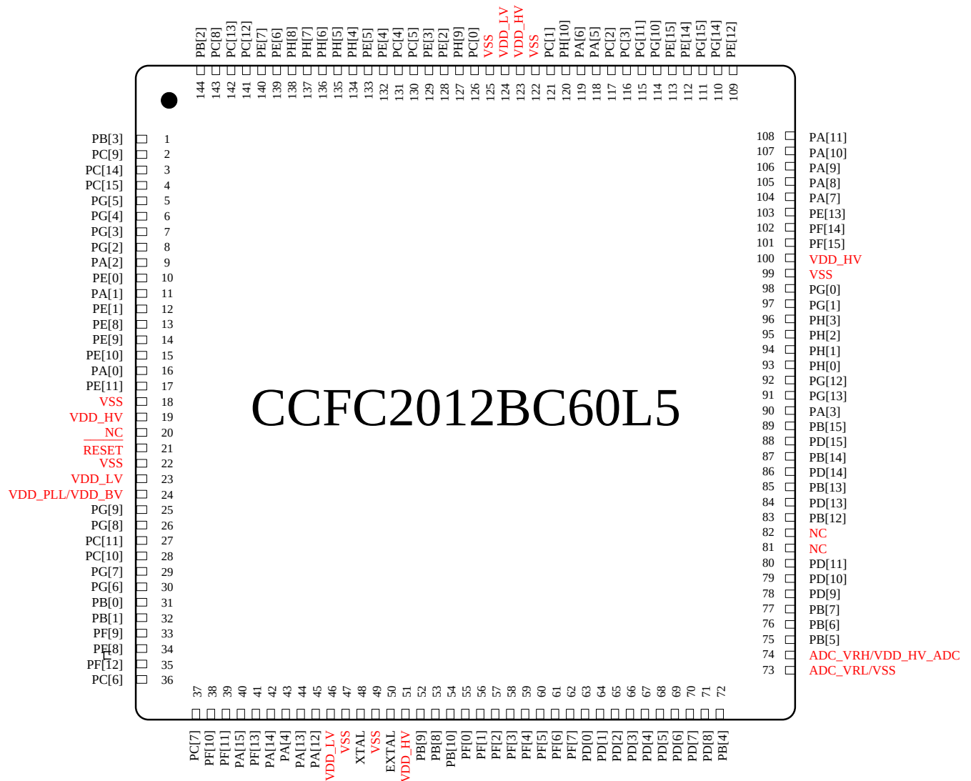
Figure 3. CCFC2012BC60L5 144 LQFP pin configuration
