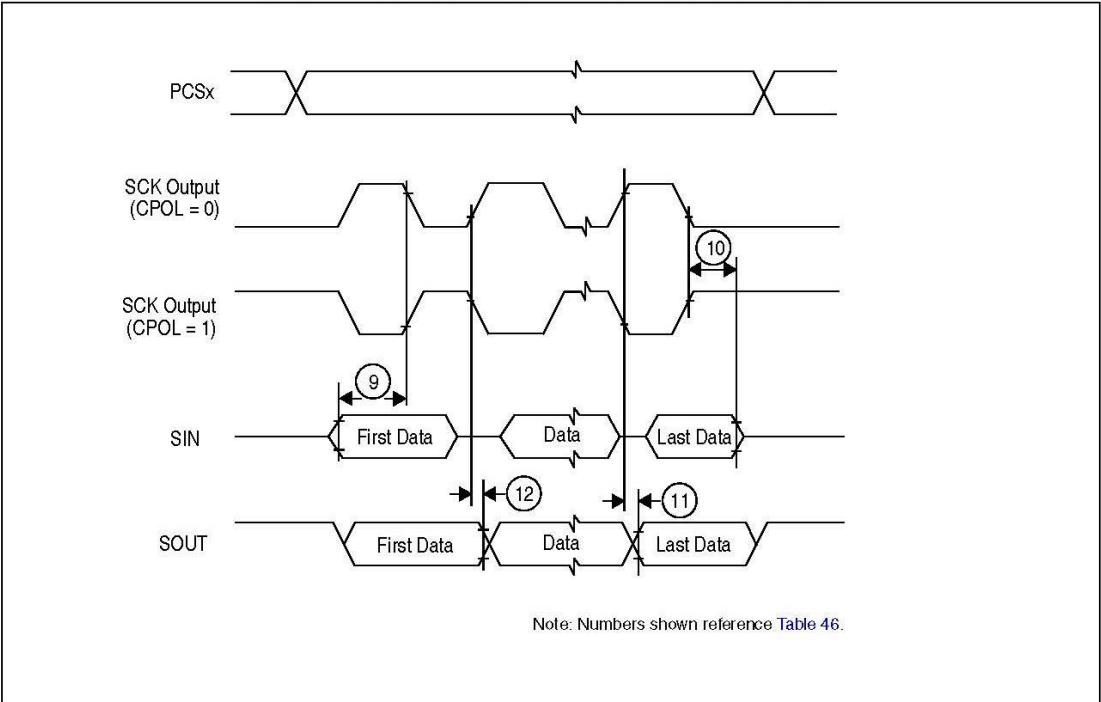
Figure 23. DSPI classic SPI timing — master, CPHA = 1
