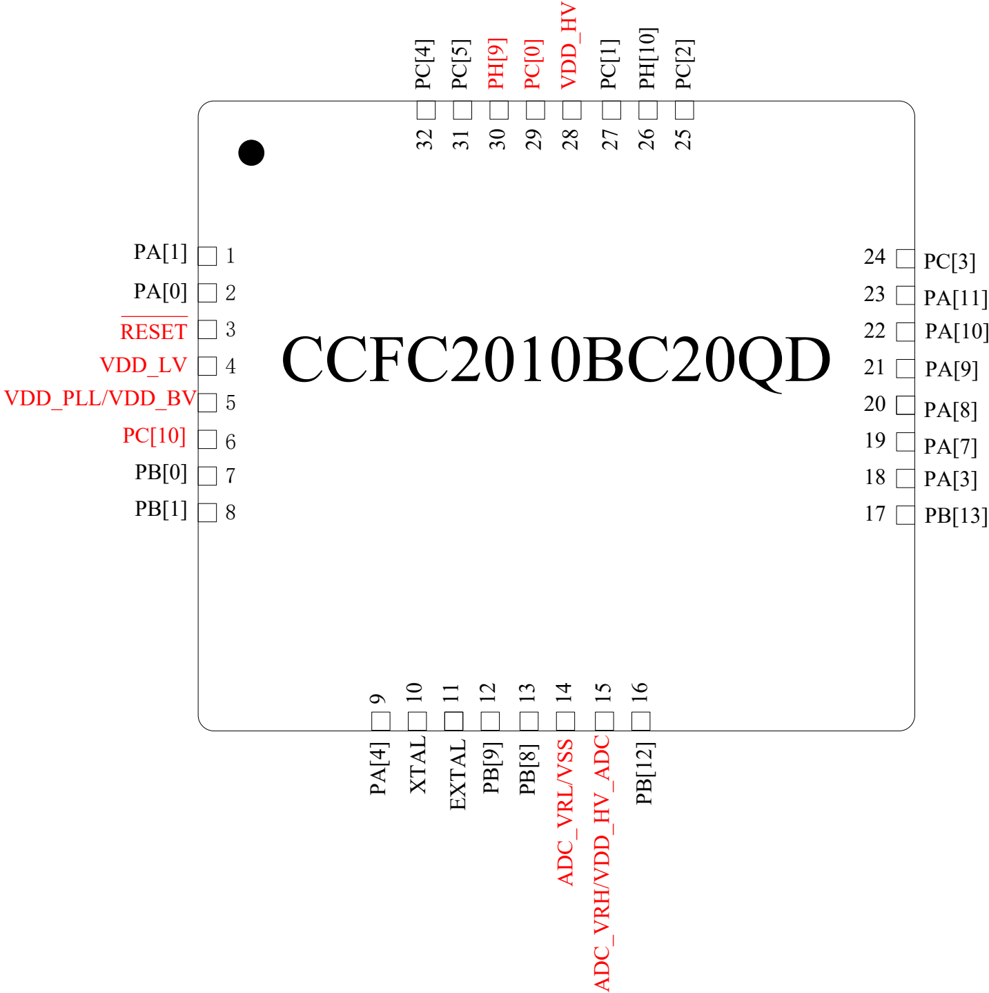
Figure 2. CCFC2010BC20QD 32-pin QFN pinout
