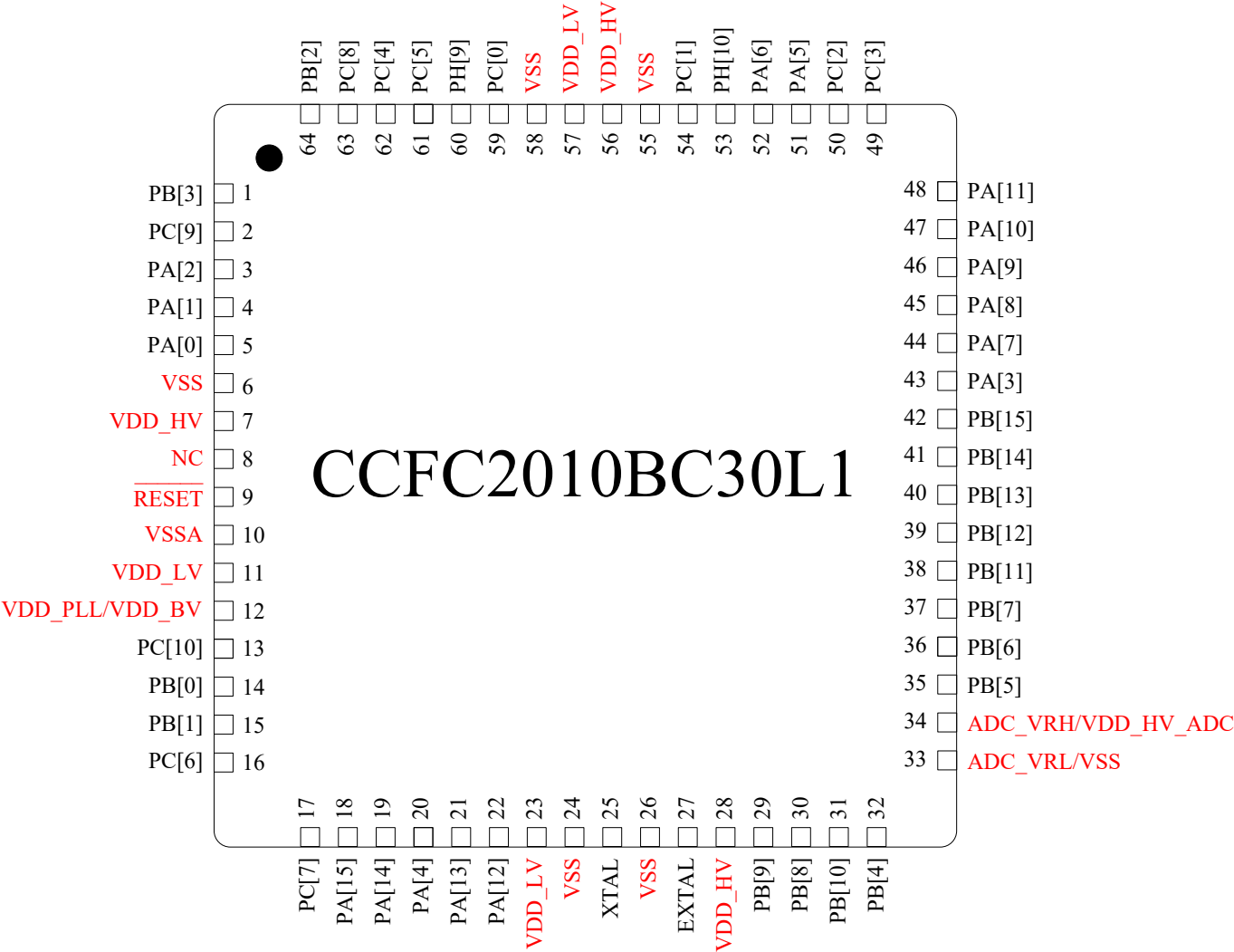
Figure 6. CCFC2010BC30L1 64-pin LQFP pinout
