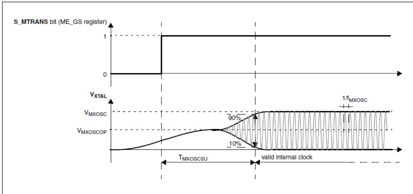
Figure 13. Fast external crystal oscillator (4 to 16 MHz) timing diagram
