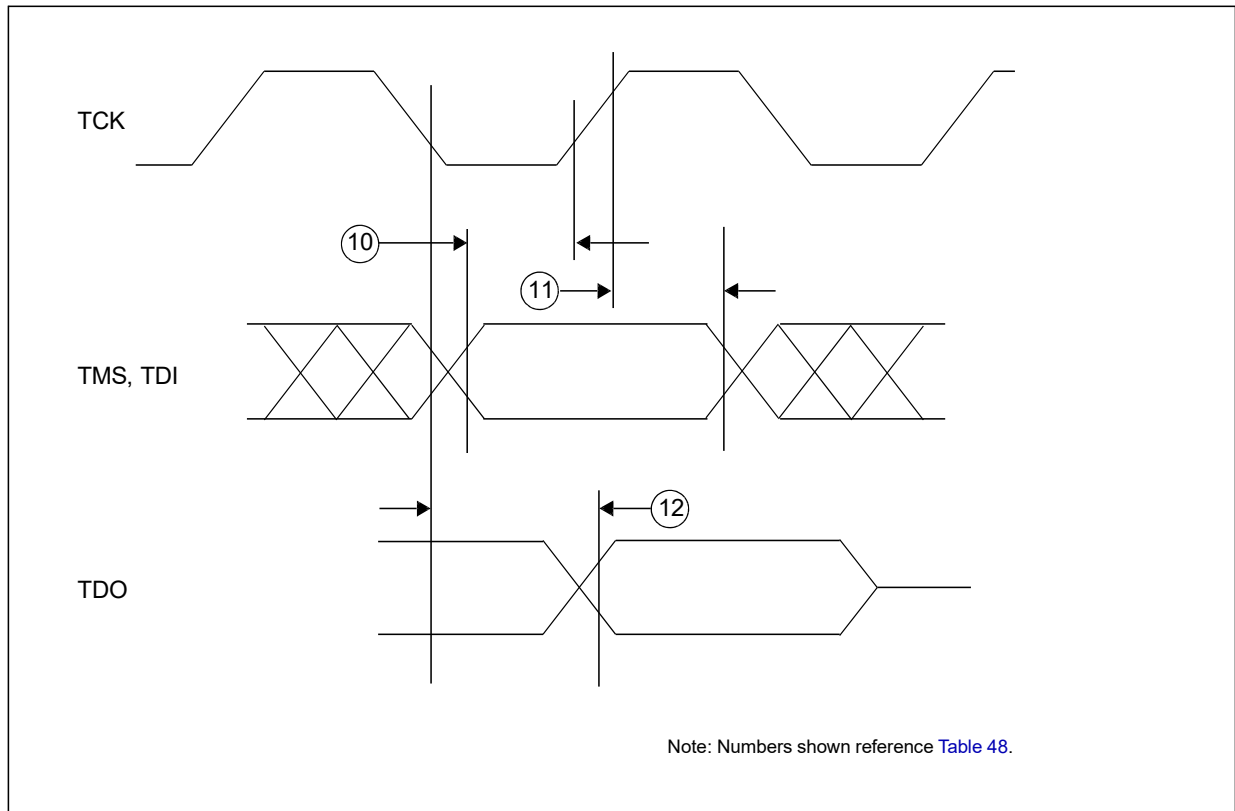
Figure 32. Nexus TDI, TMS, TDO timing
